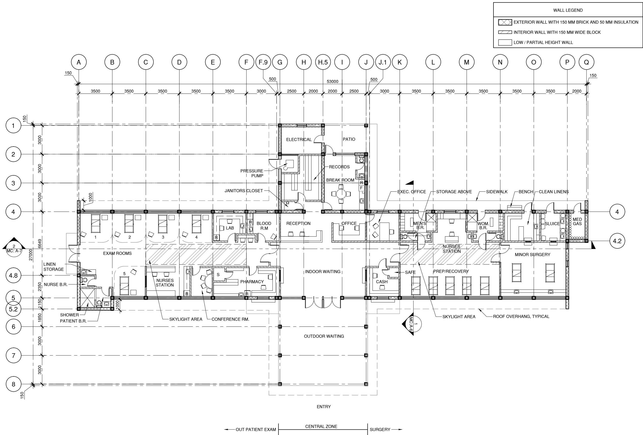
1 GROUND FLOOR PLAN WITH FURNITURE 1:200
