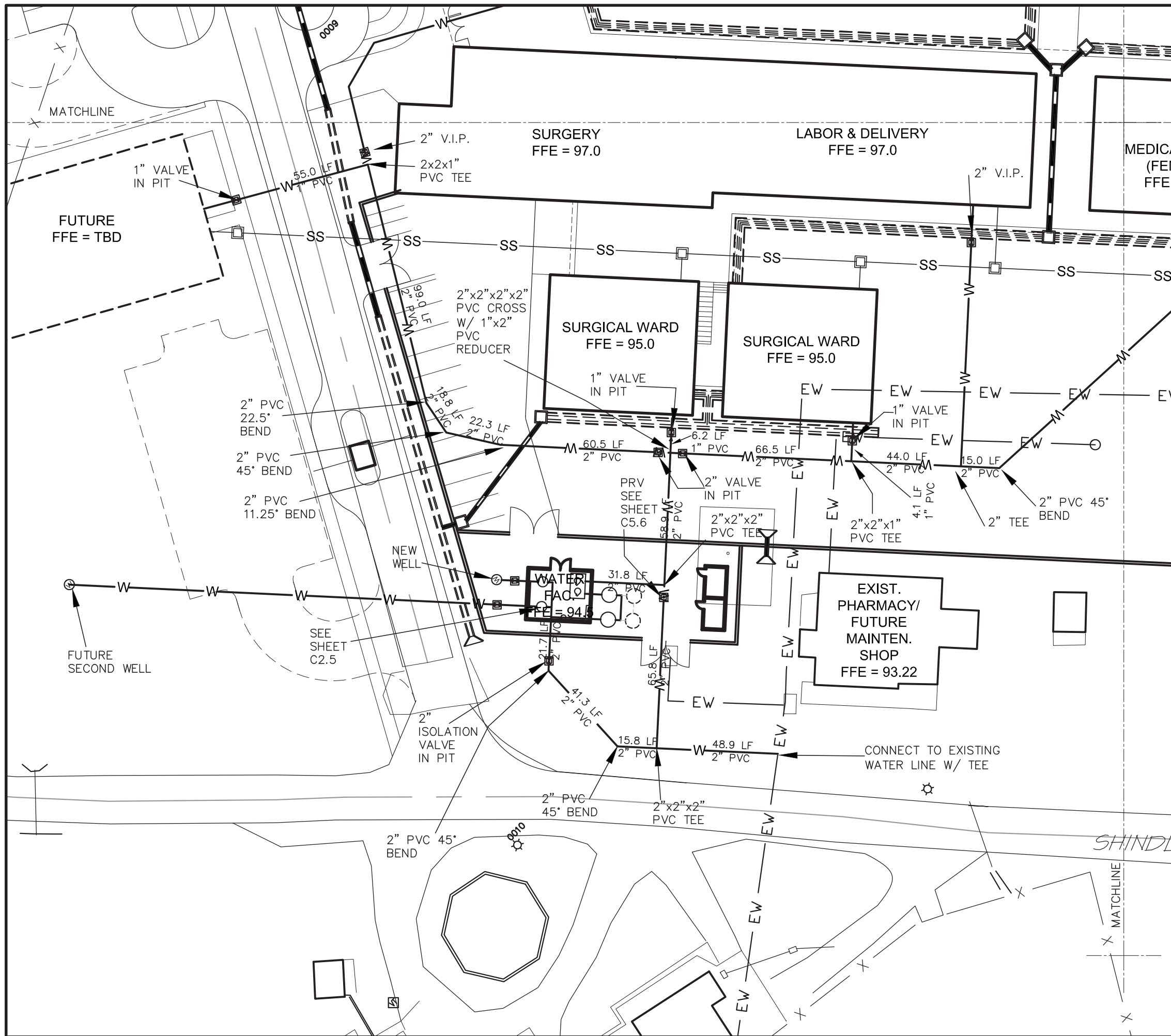
1 WATER PLAN WEST 1" = 40'-0"
