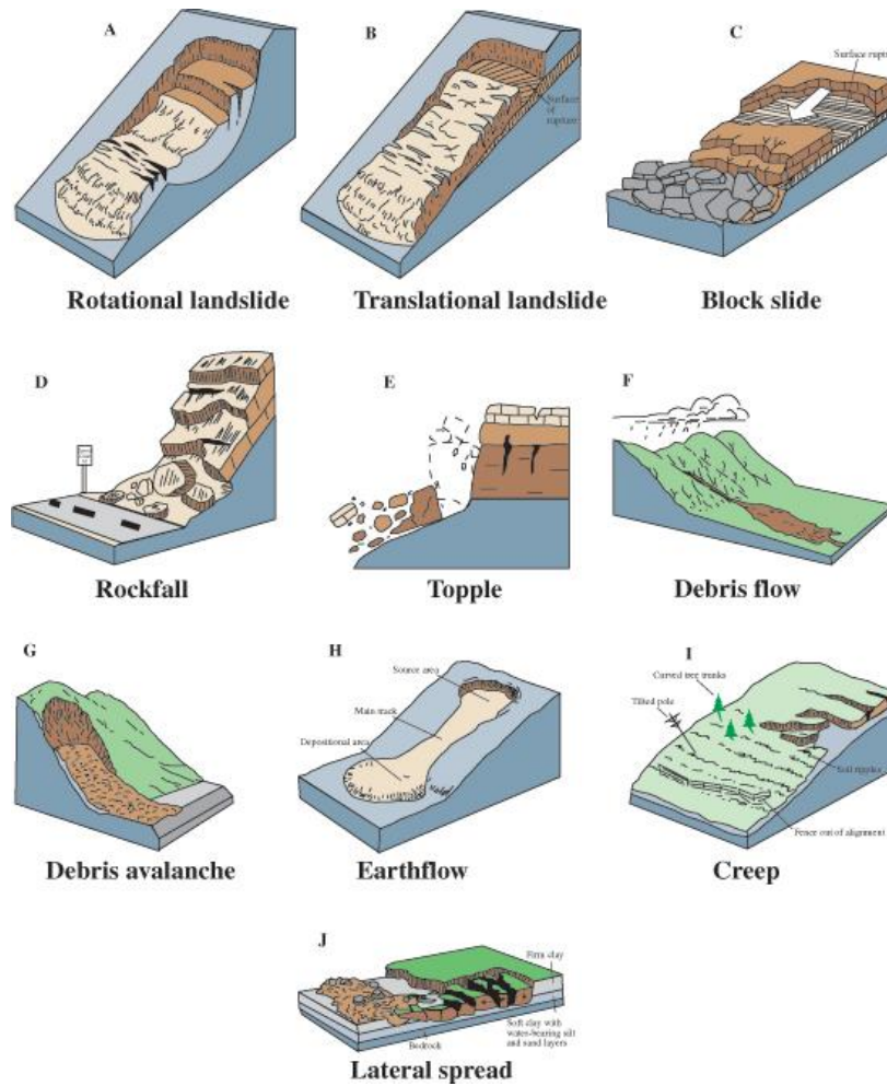
Figure 18. Types of slope failures (image from USGS 7 ).
